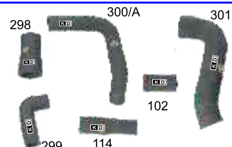
9530 ZETOR 2522/3522/4511 RAD. HOSE 298 RAD. SMALL HOSE 299 RAD. SIDE HOSE 300/A 55011310 BOTTOM HOSE 301 AIR CLEANER HOSE
