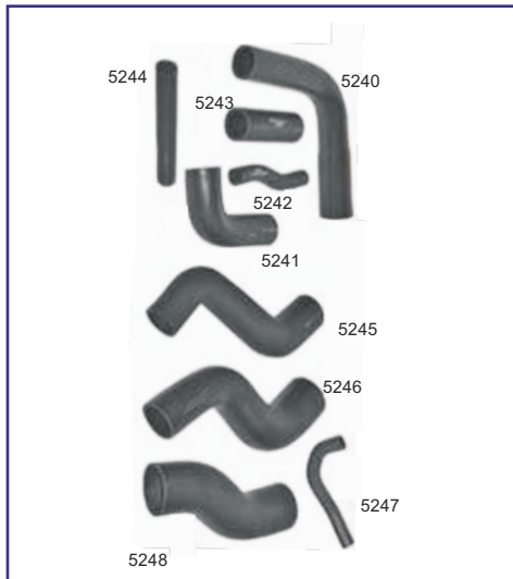
9684 TATA 709 TURBO / 1109 TURBO 5240,5241,5242,5243,5244,5245,5246,5247,5248 5240 BOTTOM (L-BEND, BIG) 5241 TOP (L-BEND, SMALL) 5242 TC OUTLET TO OIL PUMP 5243 CUT PIECE, (1 1/2" X 5") 5244 CUT PIECE, (3/4" X 10") 5245 A/C 709 TURBO Z-BEND 1 1/4" & 2 1/2" 5246 A/C 1109 TURBO Z-BEND 2 1/2" & 3" 5247 TURBO 709 TURBO EX (L-BEND) 5248 A/C 709 BUS (S-BEND) 3" & 3"
