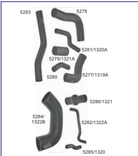
9687 TATA 407 TURBO / SPACIO / 207 Di 5277,5278,5279,5280,5281,5282,5283,5284,5285,5286 5277/1319A TOP (DOUBLE BEND) 5278 BOTTOM (L-BEND) 5279/1321A CUT PIECE, (1 1/2" X 4") 5280 NALKI (C-TYPE, SMALL) 5281/1320A NALKI (BIG) 5282/1322A ALT. SPACIO/207 DI/RX 5283 DIESEL TANK 207 DI 5284/1322B A/C SPACIO (U-BEND) 5285/1320 S-BEND 407 TURBO (SMALL) 5286/1321 BELLOW 5.75" LONG 207 DI RX
